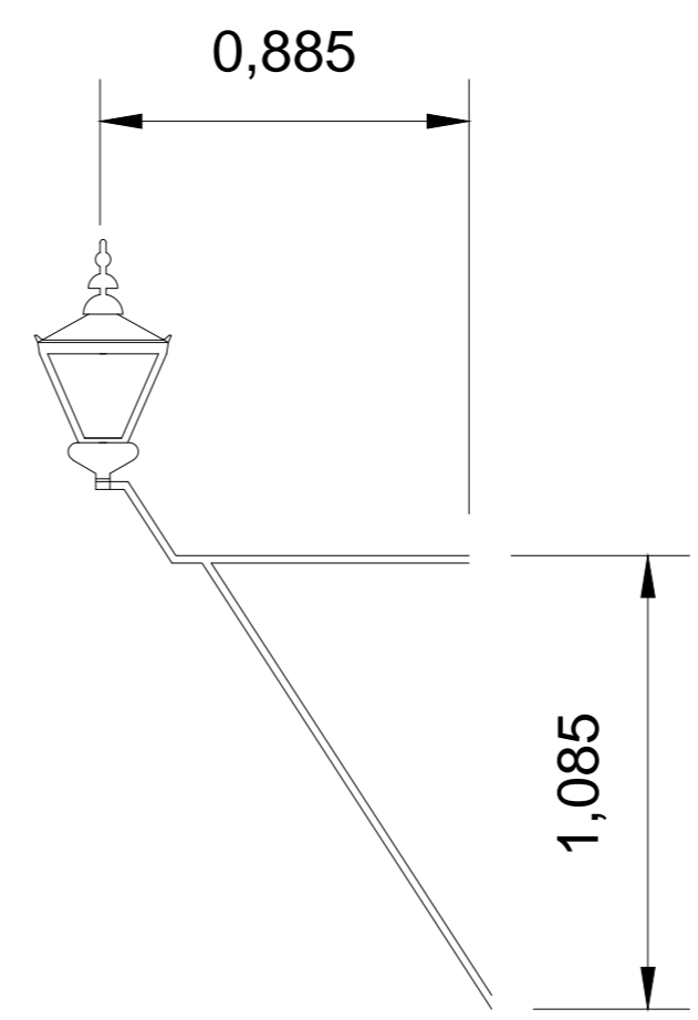
18" Windsor gas lantern on purpose made steel brackets fixed to wall. Quantity 2 No.
